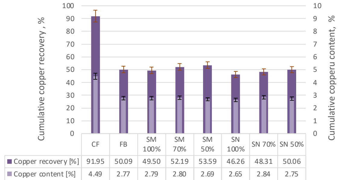
Fig. 6. Comparison of comparative flotation (CF), collectorless (FB), spruce lignin microparticles (SM), spruce lignin nanoparticles (SN)
