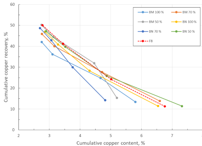
Fig. 3. Comparison of birch lignin microparticles (BM) and birch lignin nanoparticles (BN) curves
