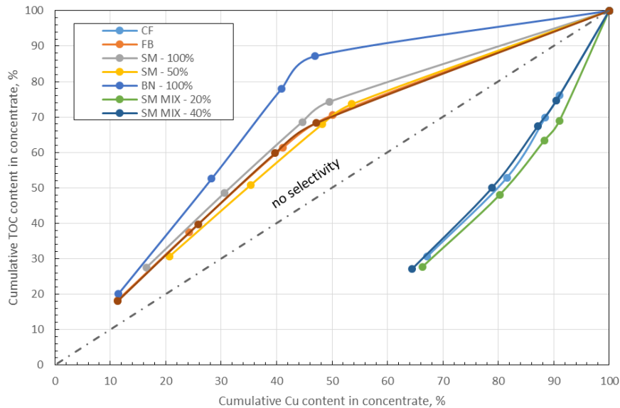
Fig. 8. Recovery of copper in concentrates vs. recovery of total organic carbon
