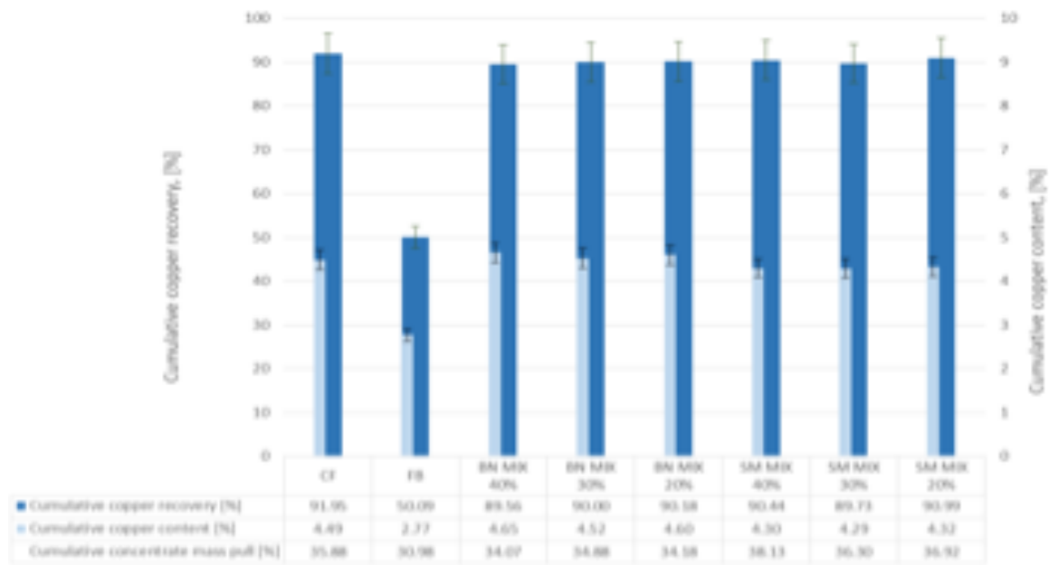
Fig. 7. Comparison of comparative flotation (CF), collectorless (FB), MIXTURES of Birch Nano (MIX BN), and MIXTURES of Spruce Micro (MIX SM)
