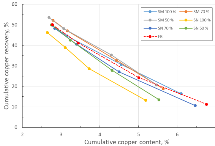
Fig. 4. Comparison of spruce lignin microparticles (SM) and spruce lignin nanoparticles (SN) curves
