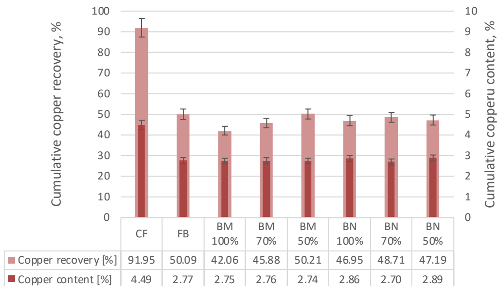
Fig. 5. Comparison of comparative flotation (CF), collectorless (FB), birch lignin microparticles (BM), birch lignin nanoparticles (BN)
