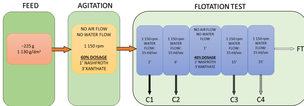
Fig. 1. Process diagram
