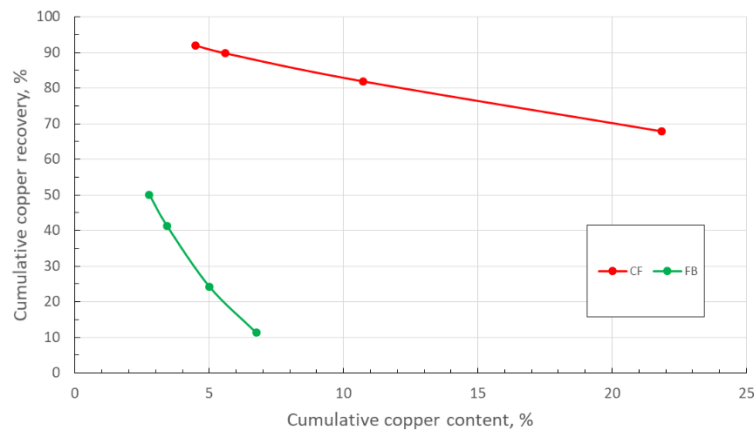
Fig. 2. Recovery-content curves for Cu: of comparative flotation (CF) and collectorless flotation (FB)
