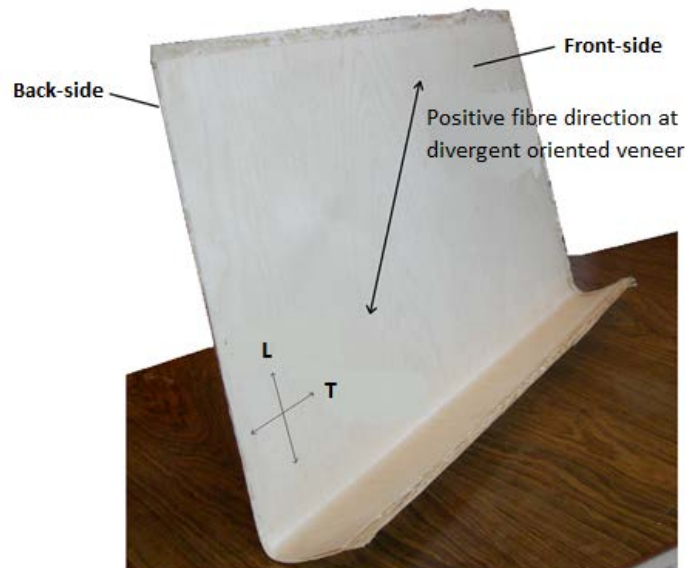
Figure 2. A shell that was studied in this investigation, with the different definitions used in this paper: front- and backside of the shell, positive fibre direction, lengthwise- and transverse direction.
