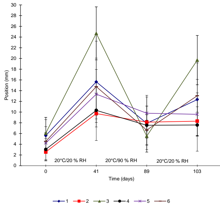
Figure 5. Mean position in shells manufactured with veneers with different fibre orientations. Test groups 1-6 according to Table 1.
