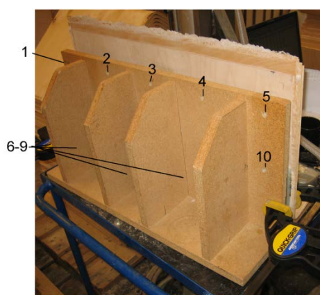
Figure 4. Gauge for measuring of shape. The numbers in the image indicates measuring the positions and designations.
