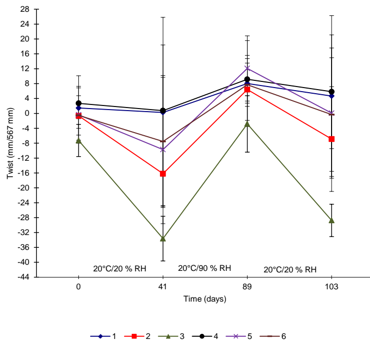
Figure 6. Mean twist in shells manufactured with veneers with different fibre orientations. Test
