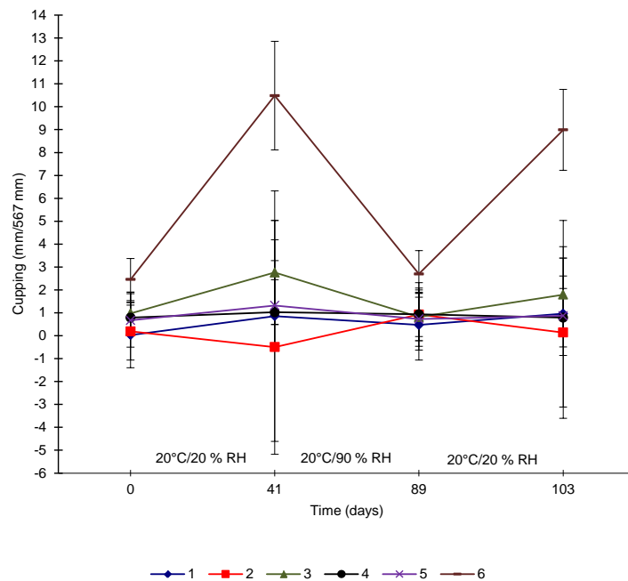
Figure 7. Mean cupping in shells manufactured with veneers with different fibre orientations. Test groups 1-6 according to Table 1.
