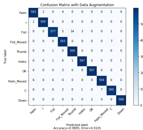
Fig. 10. Confusion Matrix of Hand Gesture Recognition Database
