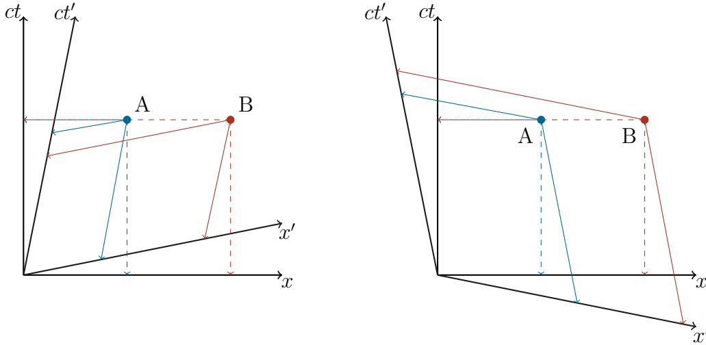
Figure 1: Minkowski diagram for measurement of entangled Bell-correlated events, A and B , simultaneous in the lab ( ct, x ), with reference frames moving inertially relative to the lab ( ct', x' ) in which A and B are non-simultaneous: Left v \approx 0.2c ( B prior to A ), Right v \approx -0.2c ( A prior to B ). This results for arbitrarily small space separation \epsilon = |x_A - x_B| and any v \neq 0 , assuming that t_A = t_B (simultaneity in the lab-data), calling “cause-effect” (which entangled event “collapses” which?) into question, especially as |t'_A - t'_B| \rightarrow \infty as v \rightarrow c : Why should the “collapse” be instantaneous only in the lab-frame, when there exist infinitely many other frames equally valid and real? Also, if thus “switching” cause-and-effect (which event is measured “first” and thus determines the other) there is no reason why the (postulated) random result in left-moving frame should be the same as that in a right-moving frame. But they must be as they are results , i.e. events in classical spacetime. This clearly shows that the “Born Rule” is nonlocal in spacetime, but does not explain why (potentially) different outcomes never occur in different frames, as the “Born Rule” is postulated to be fundamentally random. If nature instead is superdeterministic, so that results A and B are predetermined - like “pebbles” (events) fixed in the invariant 4D spacetime block - it can explain why events in all frames agree (without any “spooky action at a distance”). But that is unfortunately untestable in principle, as experimenters then would not have “free will” to choose what to measure. Then again, “free will” is not part of any known physical laws; both quantum theory and classical physics being completely deterministic, and the “Born Rule” (supposedly) random. “Free will” is probably directly related to consciousness , an unsolved (unsolvable?) enigma, apparently lying outside, or transcending, all known physical laws and even the very “scientific method” itself (of hypothesis \rightarrow tests \rightarrow better hypothesis \rightarrow new tests \rightarrow ...) which presupposes conscious scientists and thus cannot be used to neither deduce nor test consciousness.
